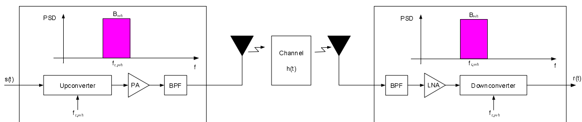
Figure 6.4 Block diagram of cognitive radio transceiver for the whole spectrum utilization.
