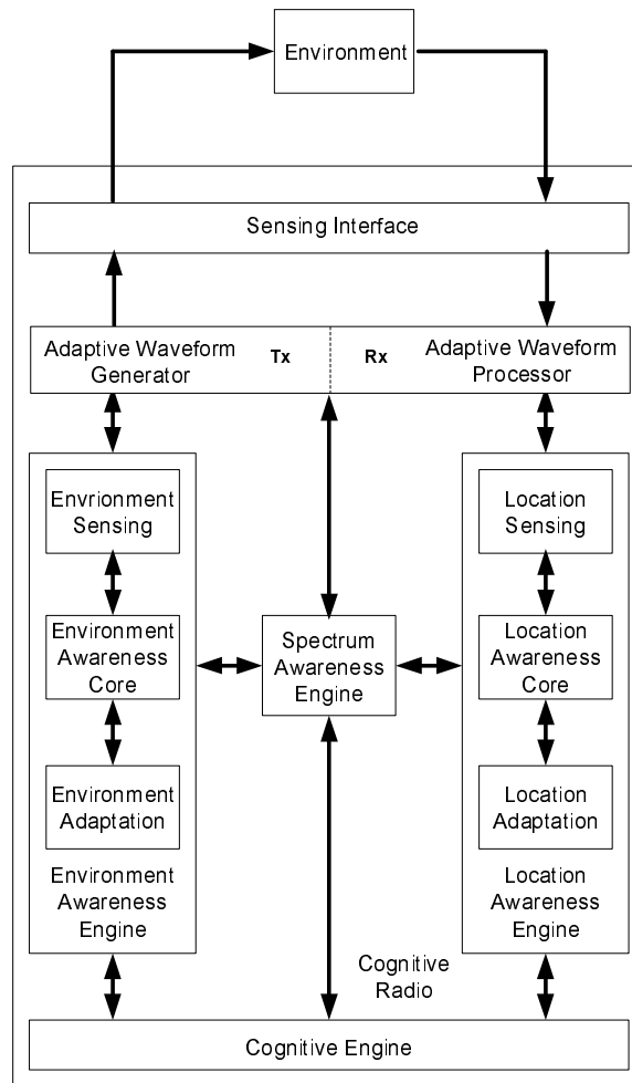
Figure 2.1 A conceptual model for cognitive radio systems with location and environment awareness cycles and engines.
