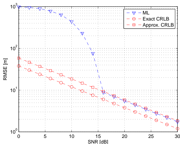
Figure 6.7 Comparison of exact and approximate CRLB for whole spectrum utilization systems.
