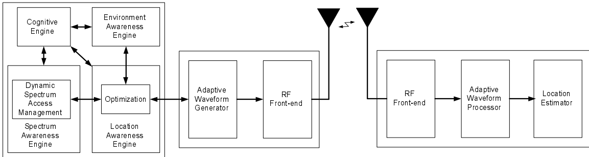
Figure 3.1 Block diagram of cognitive radio transceiver for range accuracy adaptation.
