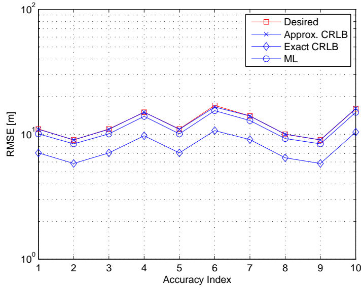
Figure 3.2 Performance of maximum likelihood range accuracy adaptation in whole spectrum utilization case.
